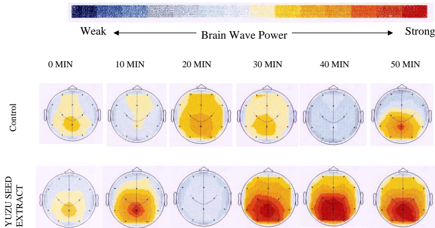
Figure 9. Brain \alpha -Wave Topography
